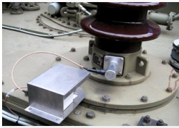
Bushing adapter
